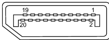
DisplayPort interface
